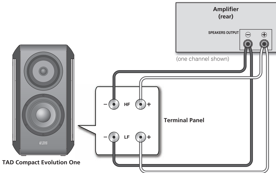
Figure 3. Connecting a TAD Compact Evolution One speaker in a bi-wired system
