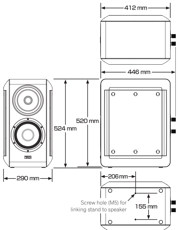
Figure 6. Overall dimensions of the TAD Compact Evolution One speaker system
