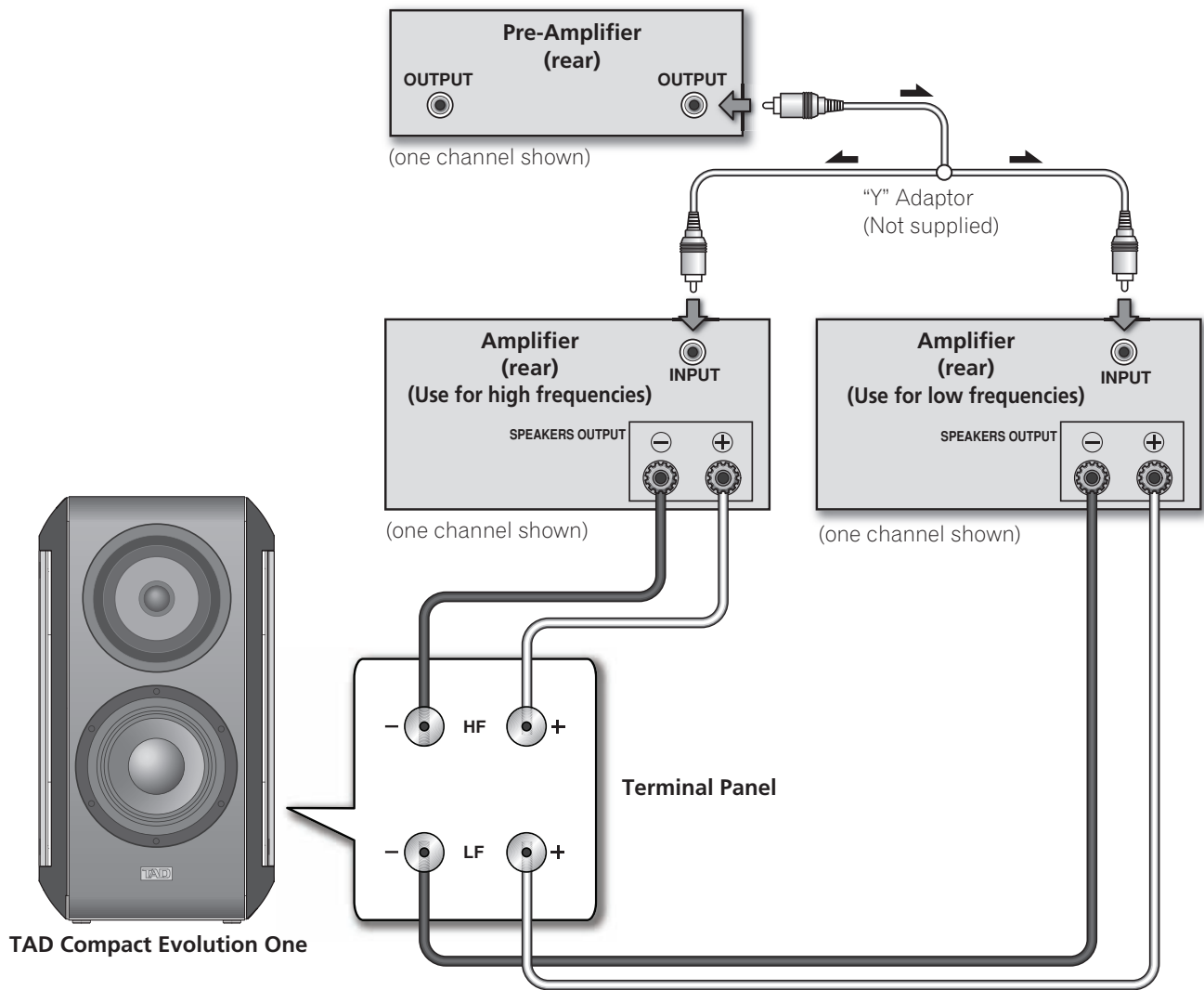
Figure 5. Connecting a TAD Compact Evolution One speaker in a horizontal bi-amplified system
