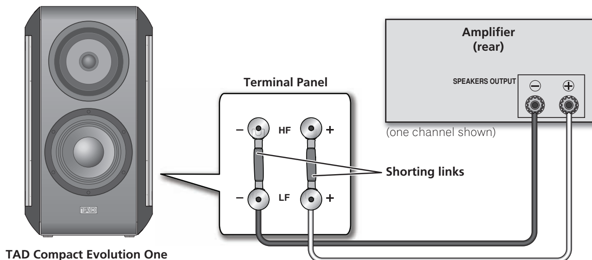
Figure 2. Connecting a TAD Compact Evolution One speaker in a single-wired system
