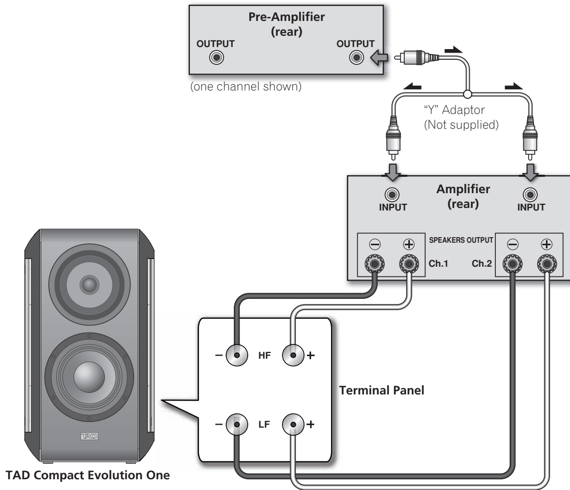
Figure 4. Connecting a TAD Compact Evolution One speaker in a vertical bi-amplified system
