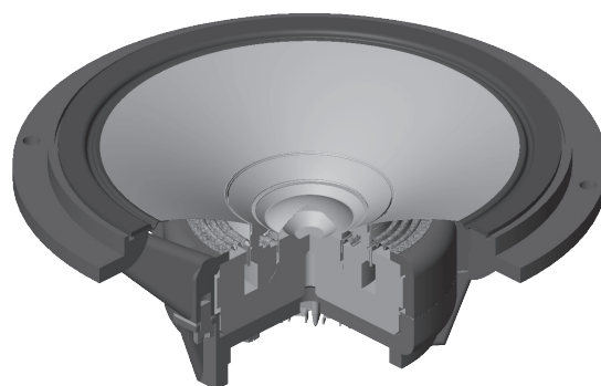
Figure 2. Le "Coherent Source Transducer" (CST) de la TAD Compact Reference
